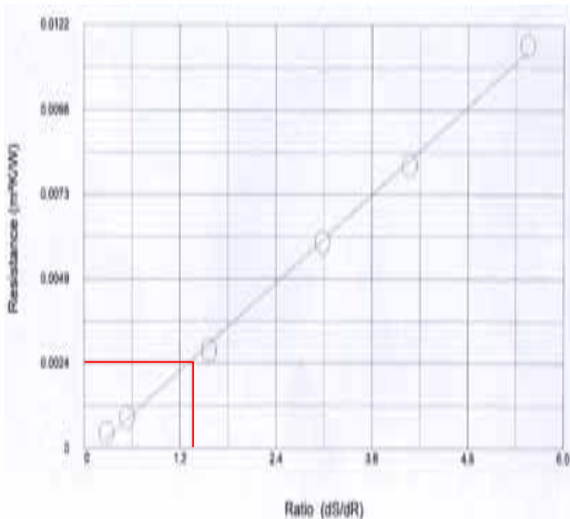
Thermal Resistance
