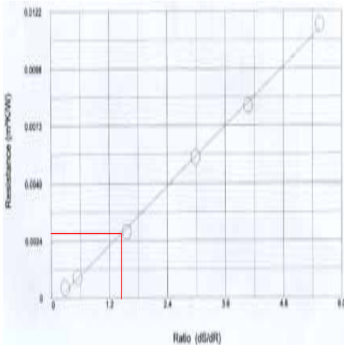
Thermal Resistance
