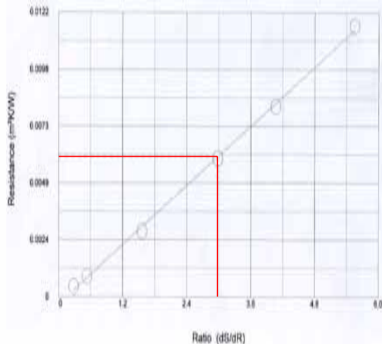
Thermal Resistance
