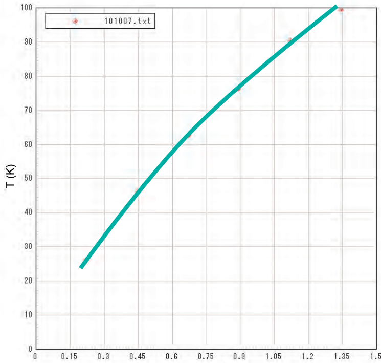
Power Consumption P (W)
