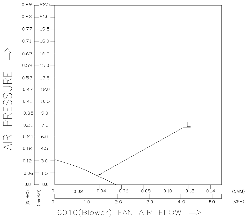
Figure 1. Fan Performance Curve
