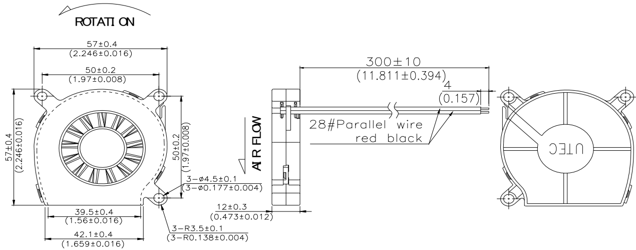
Figure 2 Fan Dimension & Assembly
