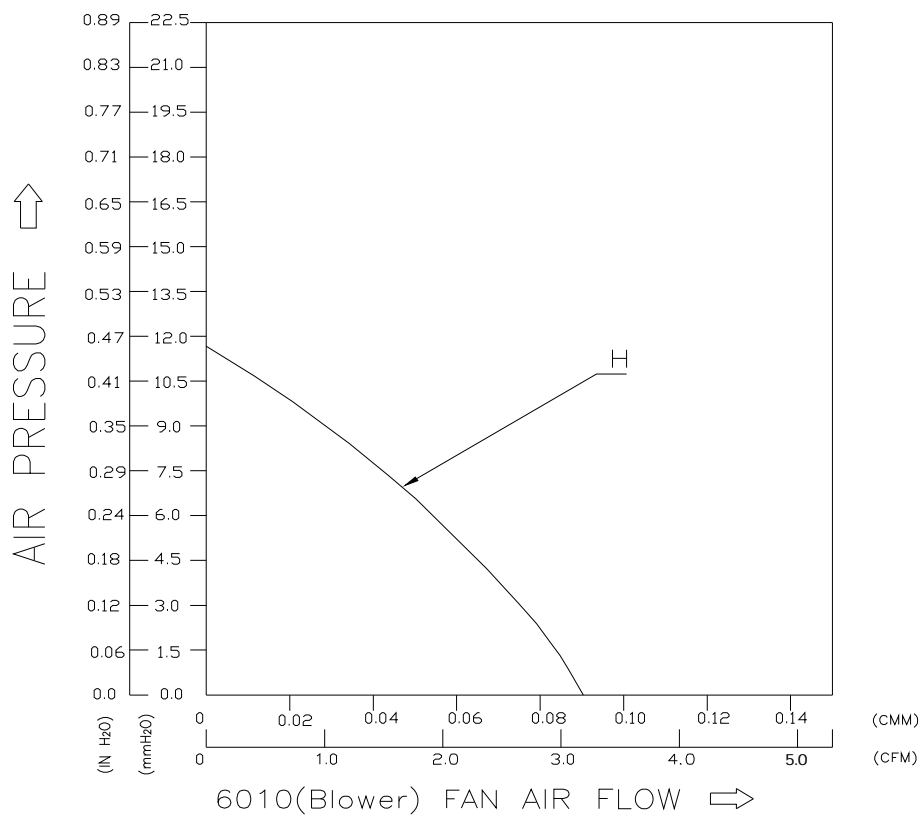
Figure 1. Fan Performance Curve
