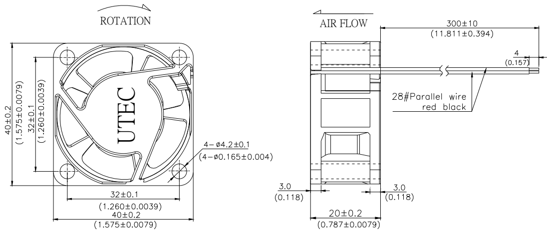
Figure 2 Fan Dimension & Assembly
