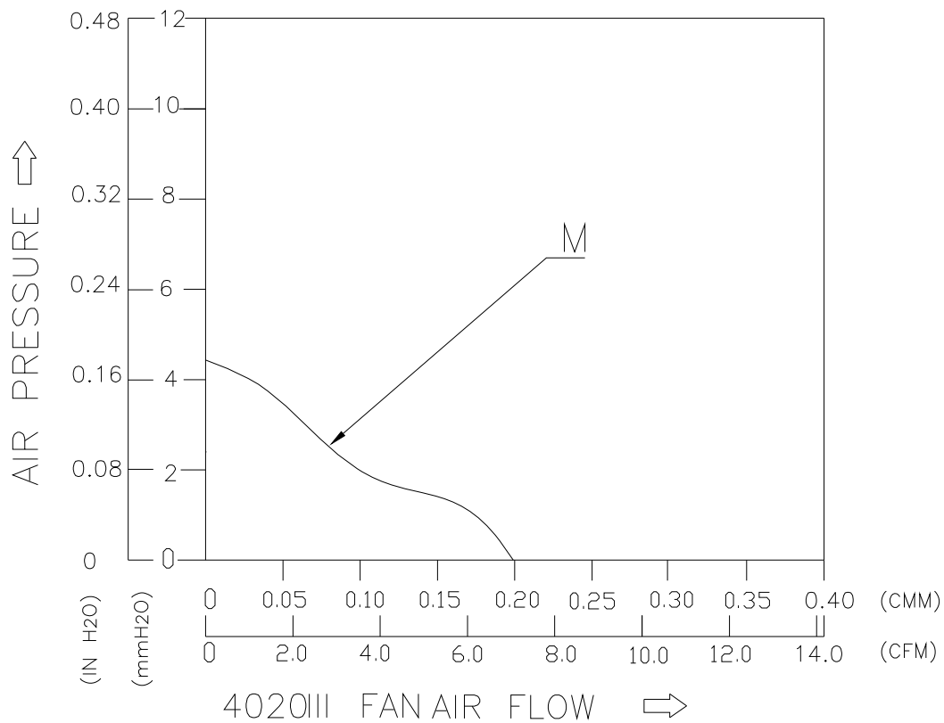
Figure 1. Fan Performance Curve
