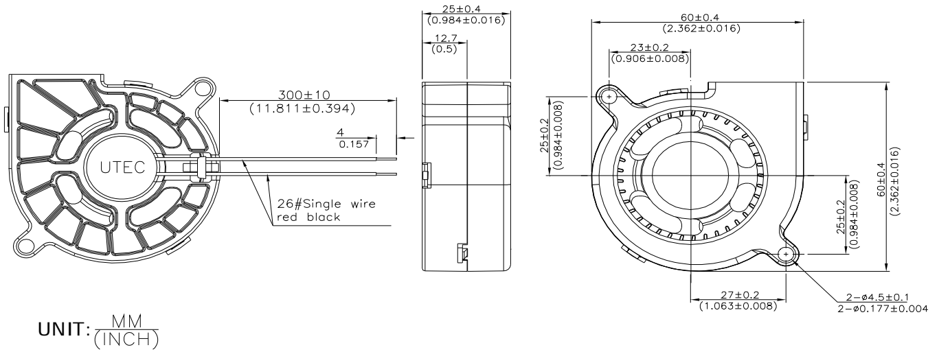
Figure 2 Fan Dimension & Assembly
