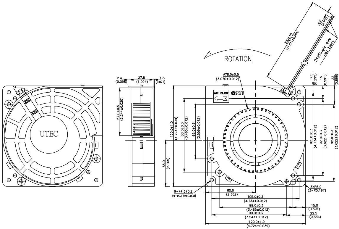
Figure 2 Fan Dimension & Assembly
