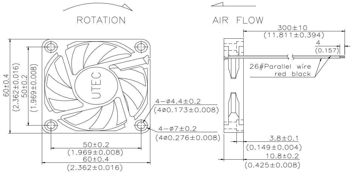
Figure 2 Fan Dimension & Assembly
