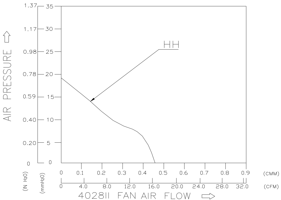
Figure 1. Fan Performance Curve
