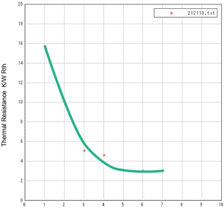
Air Speed (M/S) Forced Air Characteristics
